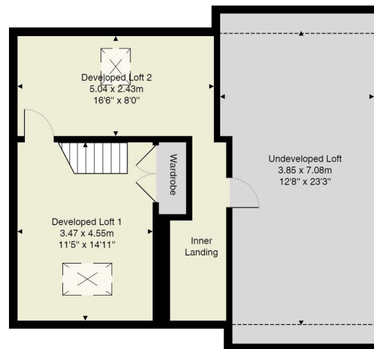
1st Floor/Loft
